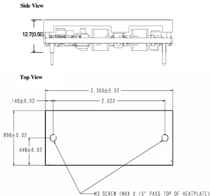
Figure 24. Converter with optional baseplate
