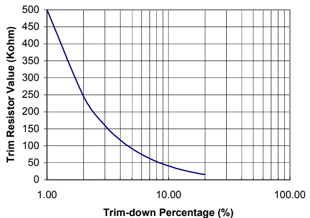
Fig. 18 Trim-Down Resistor Selection
