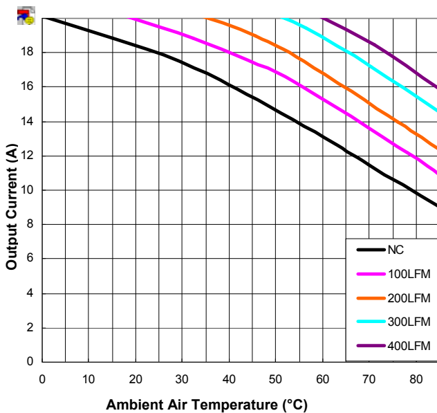
Figure 13. Current Derating Curve for Airflow Direction 2 (Ref. Fig. 14 for Airflow Direction; typical Vin, open frame unit)
