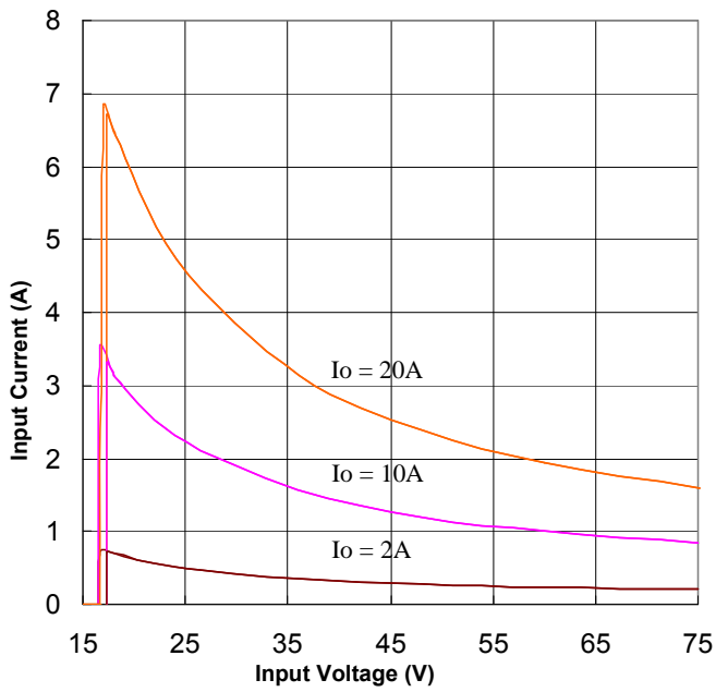
Figure 9. Input Characteristics
