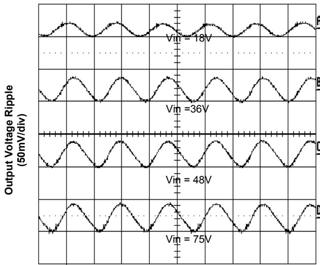
Time - t (2µs/div) Figure 5. Output Ripple Voltage at Full Load
