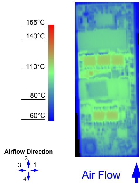
Figure 14. Thermal Image for Airflow Direction 2 (17.5A output, 55°C ambient, 200 LFM, typical Vin)
