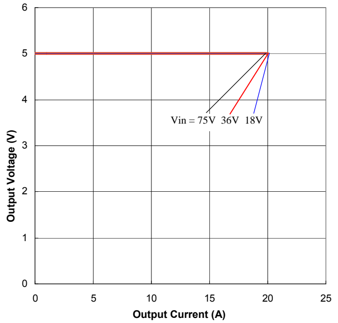
Figure 10. Output Characteristics
