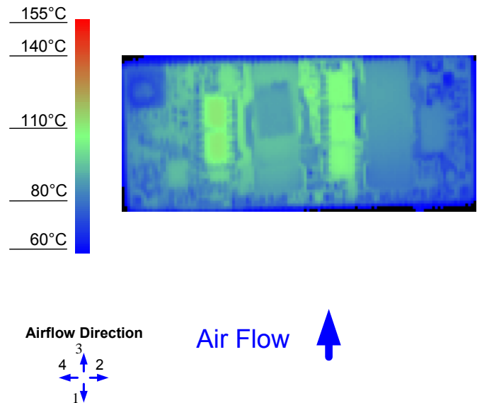
Figure 12. Thermal Image for Airflow Direction 3 18.2A output, 55°C ambient, 200 LFM, typical V_{in}
