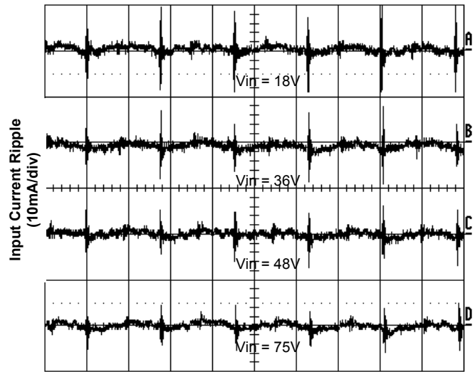
Time - t (2µs/div) Figure 6. Input Reflected Ripple Current at Full Load
