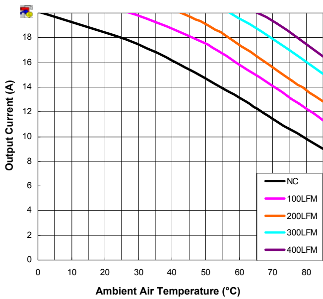
Figure 11. Current Derating Curve for Airflow Direction 3 (Ref. Fig. 12 for Airflow Direction; typical V_{in} , open frame unit)
