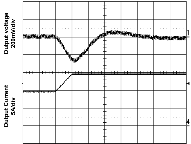
Time - t (50µs/div) Figure 8. Transient Load Response
