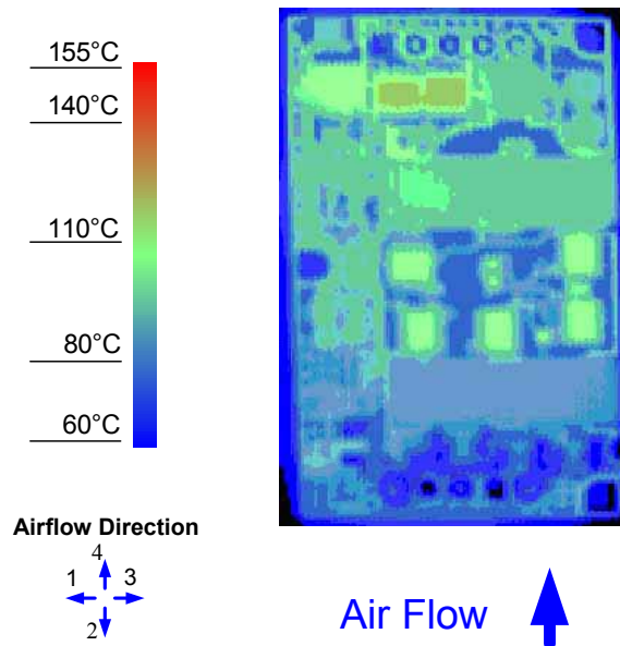
Figure 14. Thermal Image for Airflow Direction 4 (15.1A output, 55°C ambient, 200 LFM, Vin = 24V open frame unit using solder interface)
