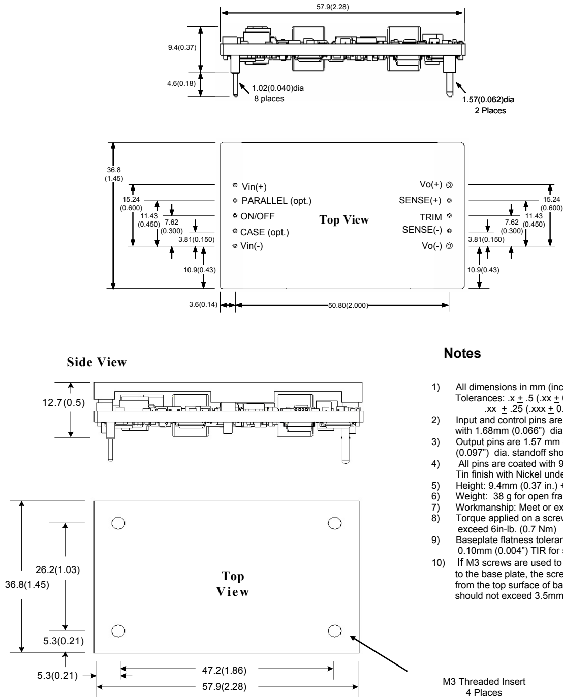
Figure 25. Converter with Optional Baseplate
