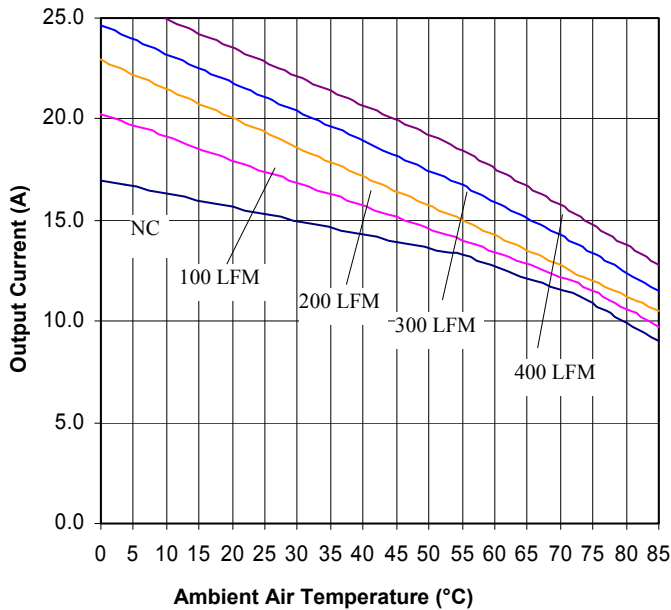
Figure 13. Current Derating Curve for Airflow Direction 4 (Ref. Fig. 14 for Airflow Direction; Vin = 24V open frame unit using socket interface)
