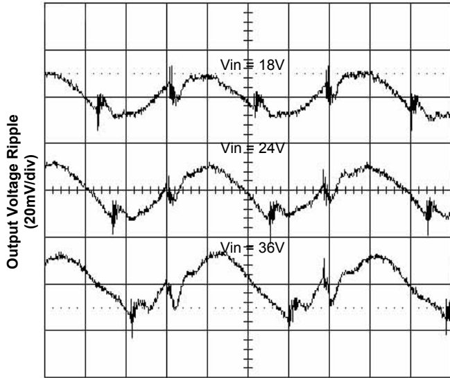
Time - t (1 \mu s/div) Figure 5. Output Ripple Voltage at 25A Load
