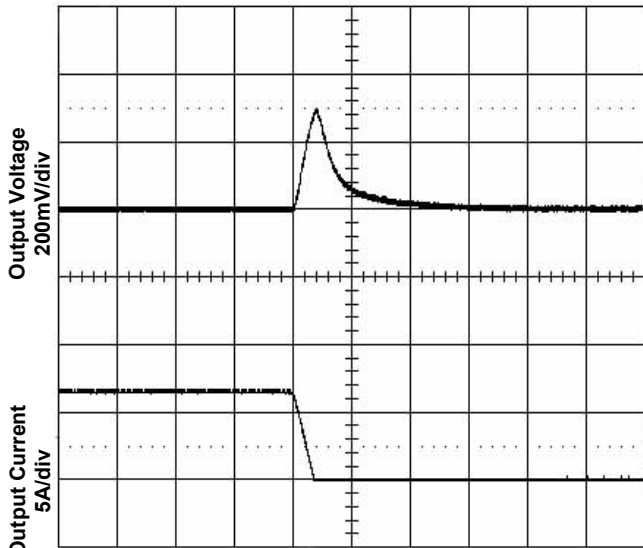
Time - t (200 \mu s/div) Figure 7. Transient Load Response
