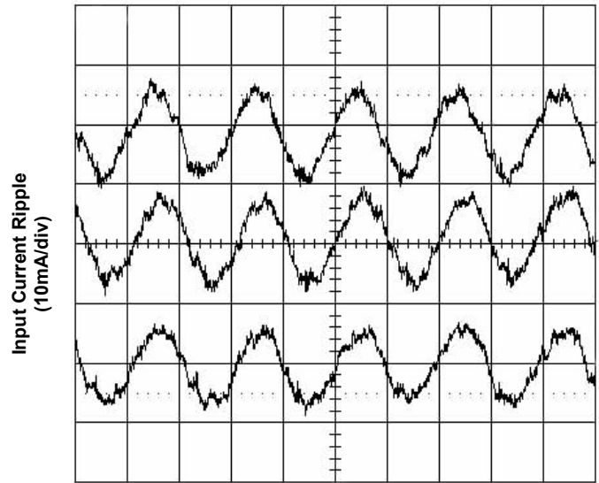
Time - t (2 \mu s/div) Figure 6. Input Reflected Ripple Current at 25A Load
