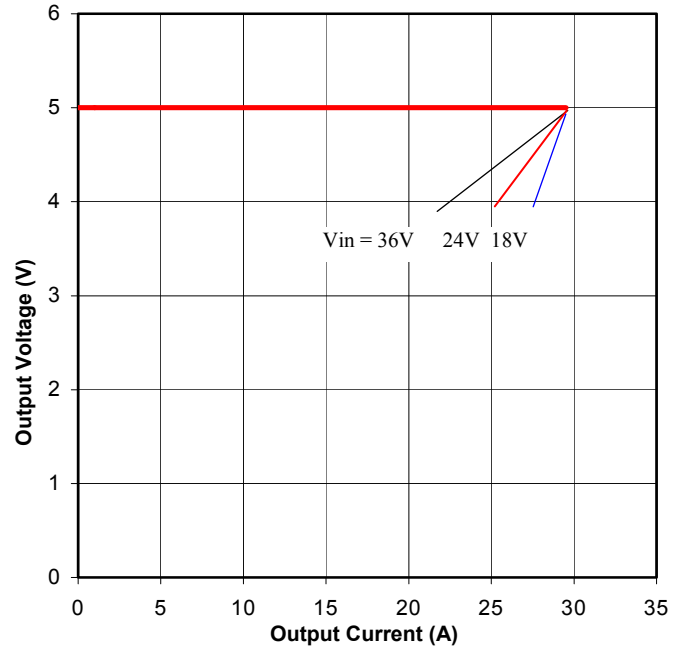
Figure 10. Output Characteristics
