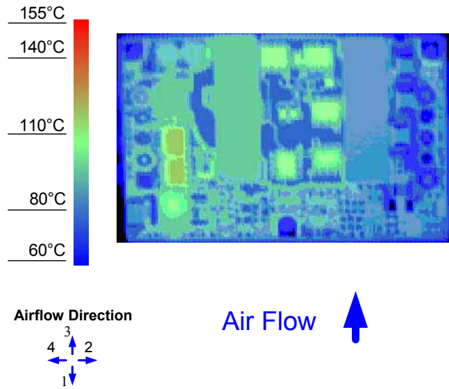
Figure 12. Thermal Image for Airflow Direction 3 (17A output, 55°C ambient, 200 LFM, V_{in} = 24V open frame unit using socket interface)
