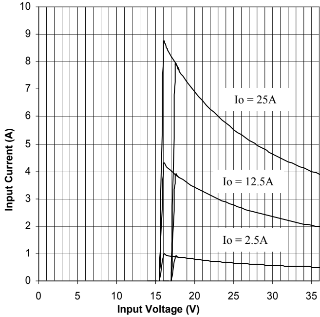
Figure 9. Input Characteristics
